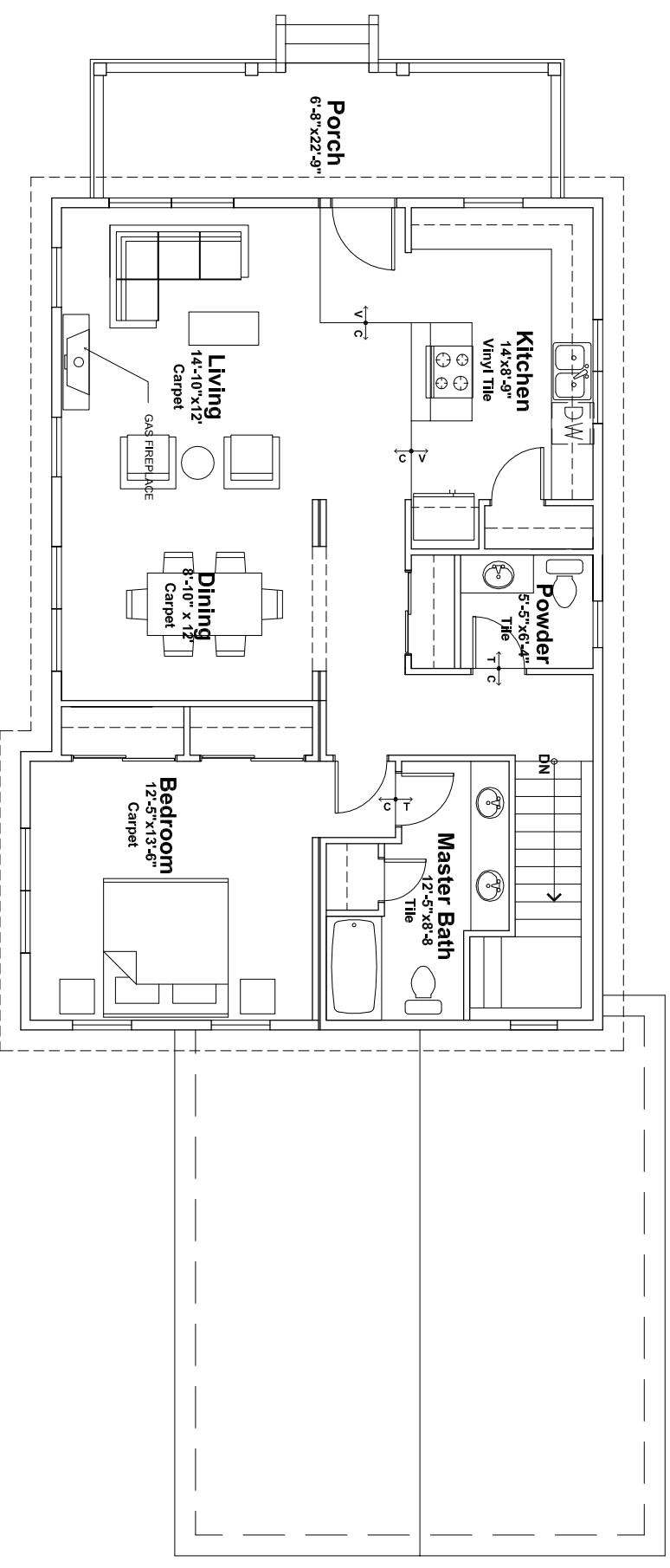
Upper Floor
